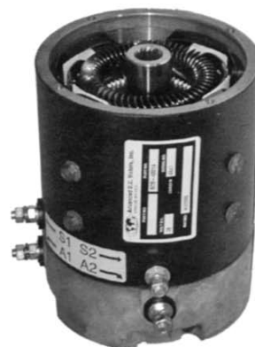
Fleet speed motor for DCS cars
